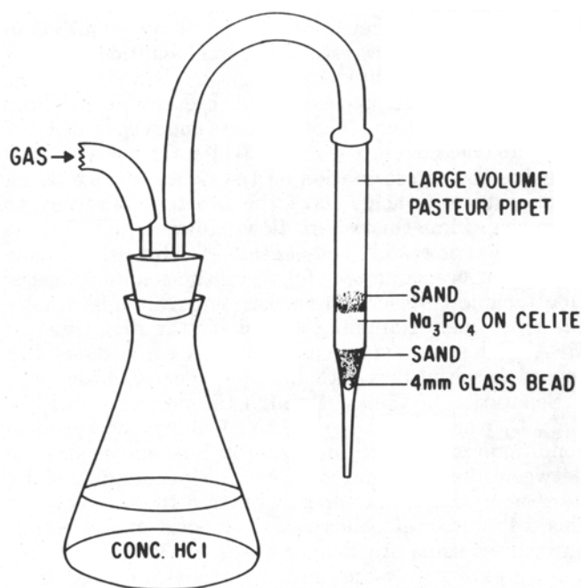
FIG. 1. Set-up for neutralizing \text{Na}_3\text{PO}_4 bed with HCl vapor.
